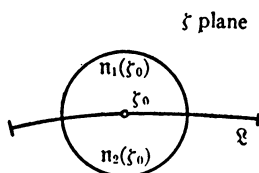
FIG. 1. The neighborhood n(\zeta) of a point \zeta_0 .
